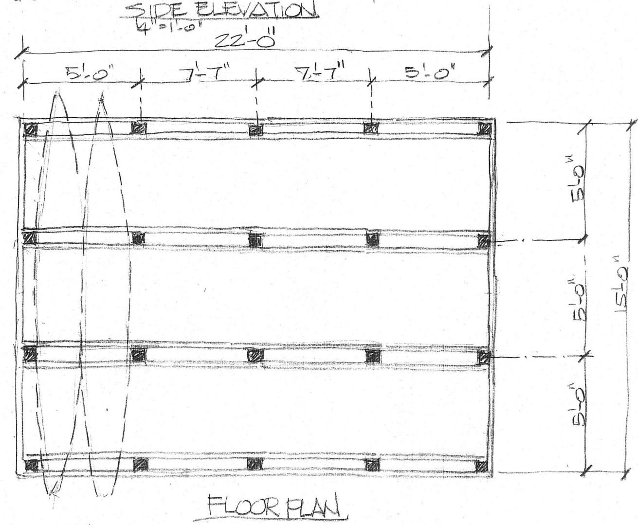
A A-2 STORAGE "A" PLANS 4"=1'-0"
