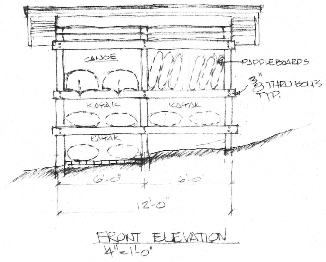
B A-2 STORAGE "B" PLANS 4"=1'-0"
